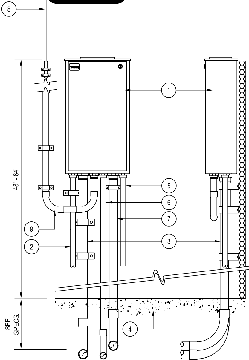
FRONT SECTION/ELEVATION NOT TO SCALE
