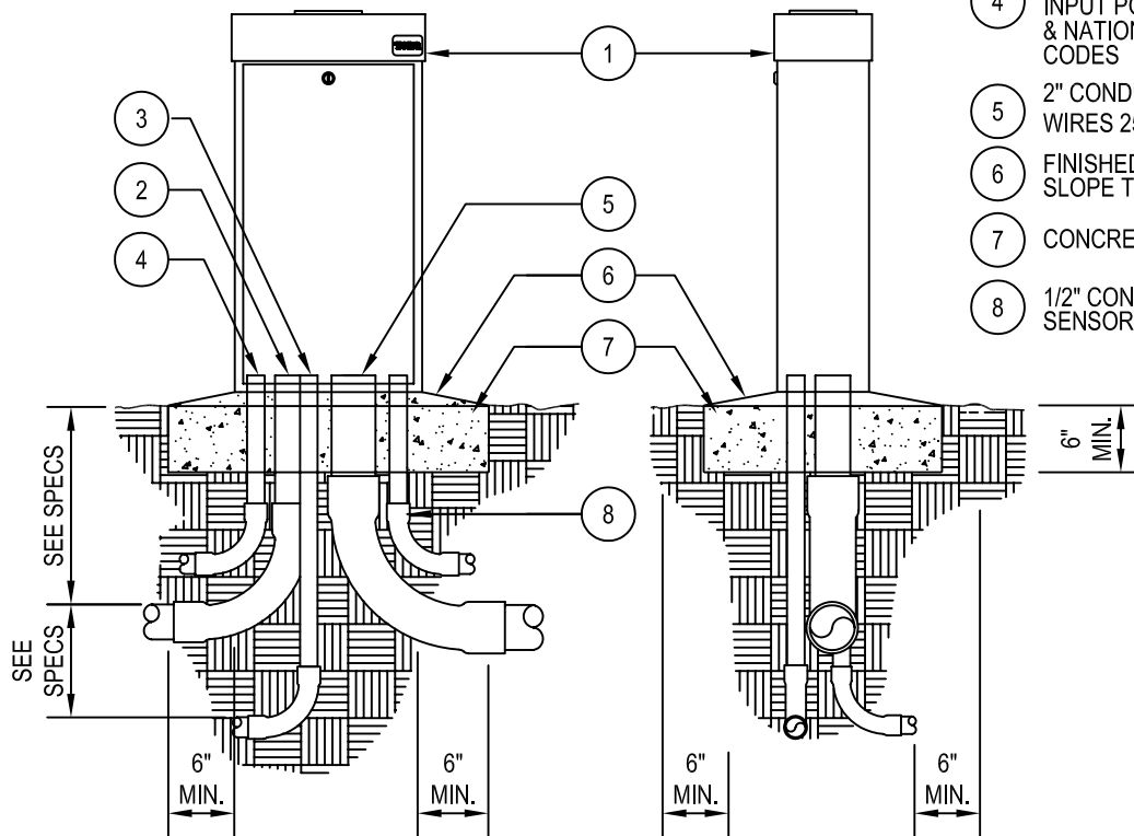
FRONT SECTION/ELEVATION NOT TO SCALE
